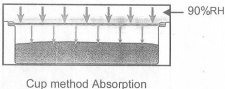
Fig 1. Desiccant Method
